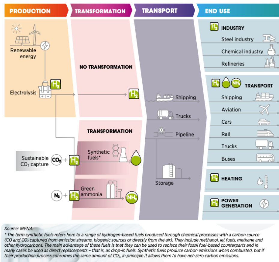
Figure 11.5: Green hydrogen production, conversion, and end uses across the energy system
